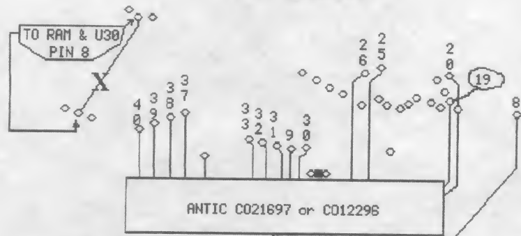
800XL ALTERNATE HOOK UP POINTS VIEW FROM TOP
